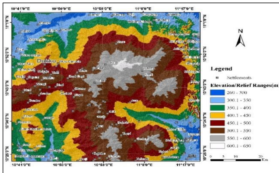
Figure 2: Elevation of Wawa Zange
